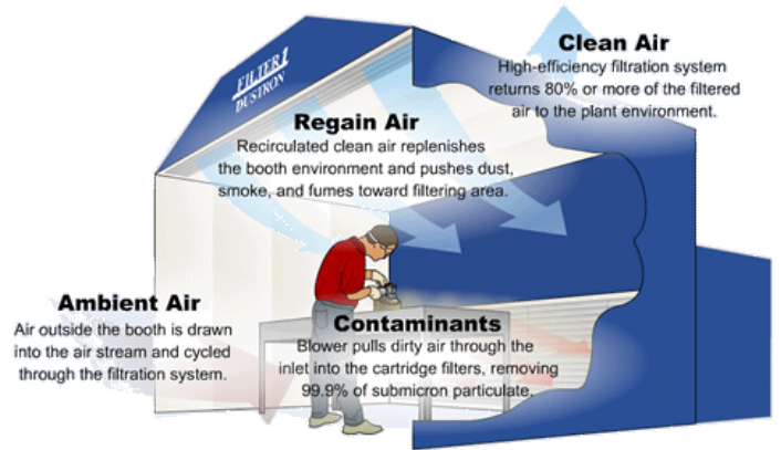
Fume Collector
